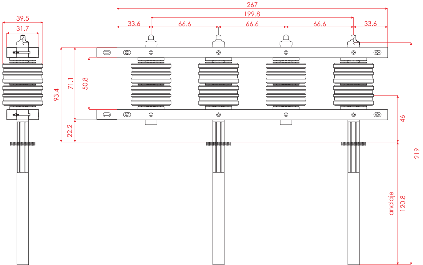
VISTA FRONTAL
