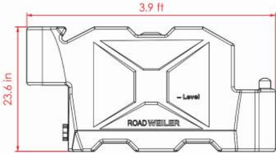
LATERAL VIEW
